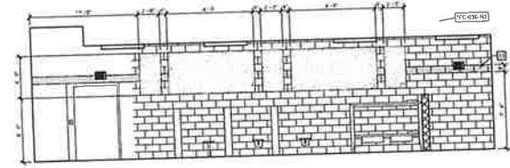
2 INTERIOR ELEVATION A2.18 A2.23 10' x 10'
